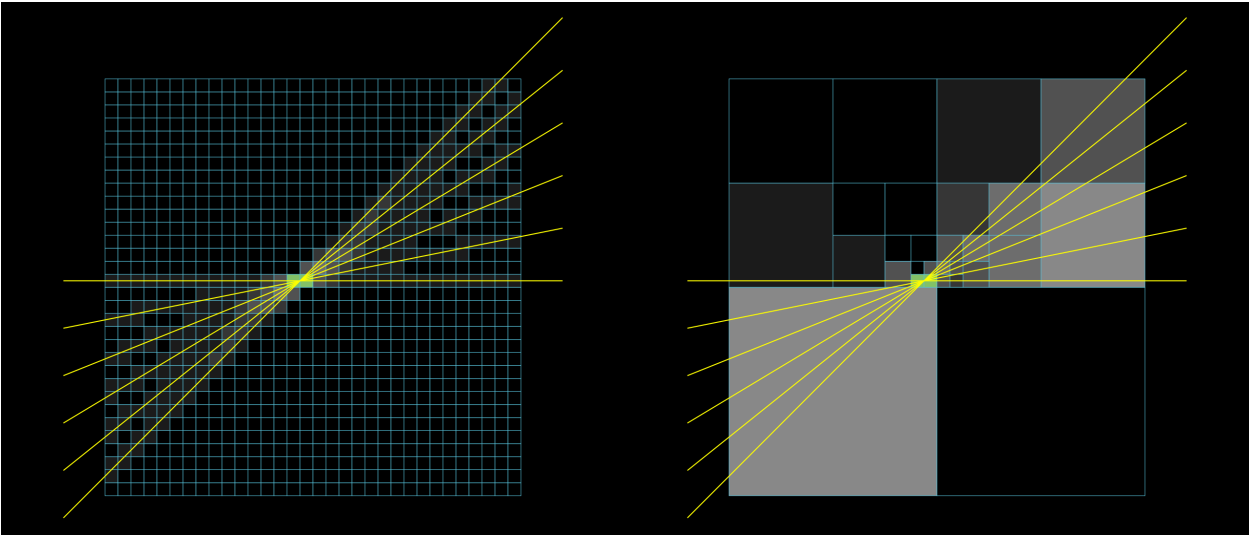
Figure 13: Traditional (left) and adaptive (right) accumulator filled with 6 points. Both accumulators have 32 cell resolution in each dimension and yield identical results.
