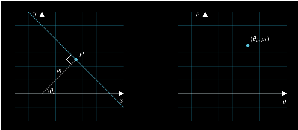
Figure 7: Line in original and Hough space.
