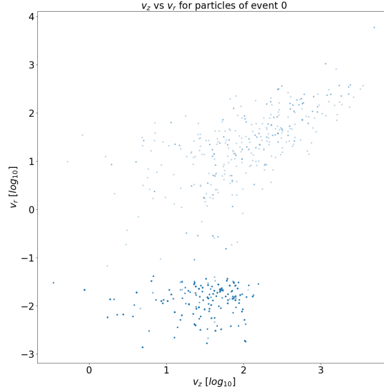
Figure 4: Distribution of v_r and v_z for particles of event 0.
