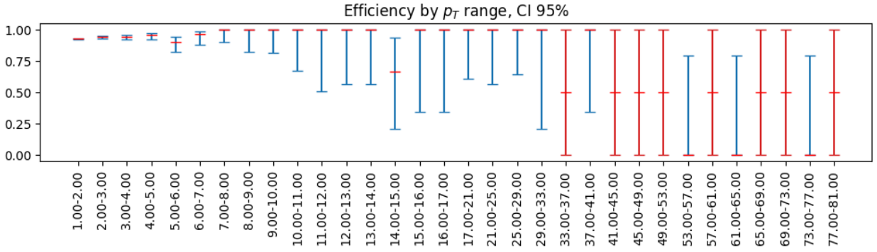
Figure 42: S test: efficiency for custom hits thresholds and lines crossing threshold 4 by p_T range.
