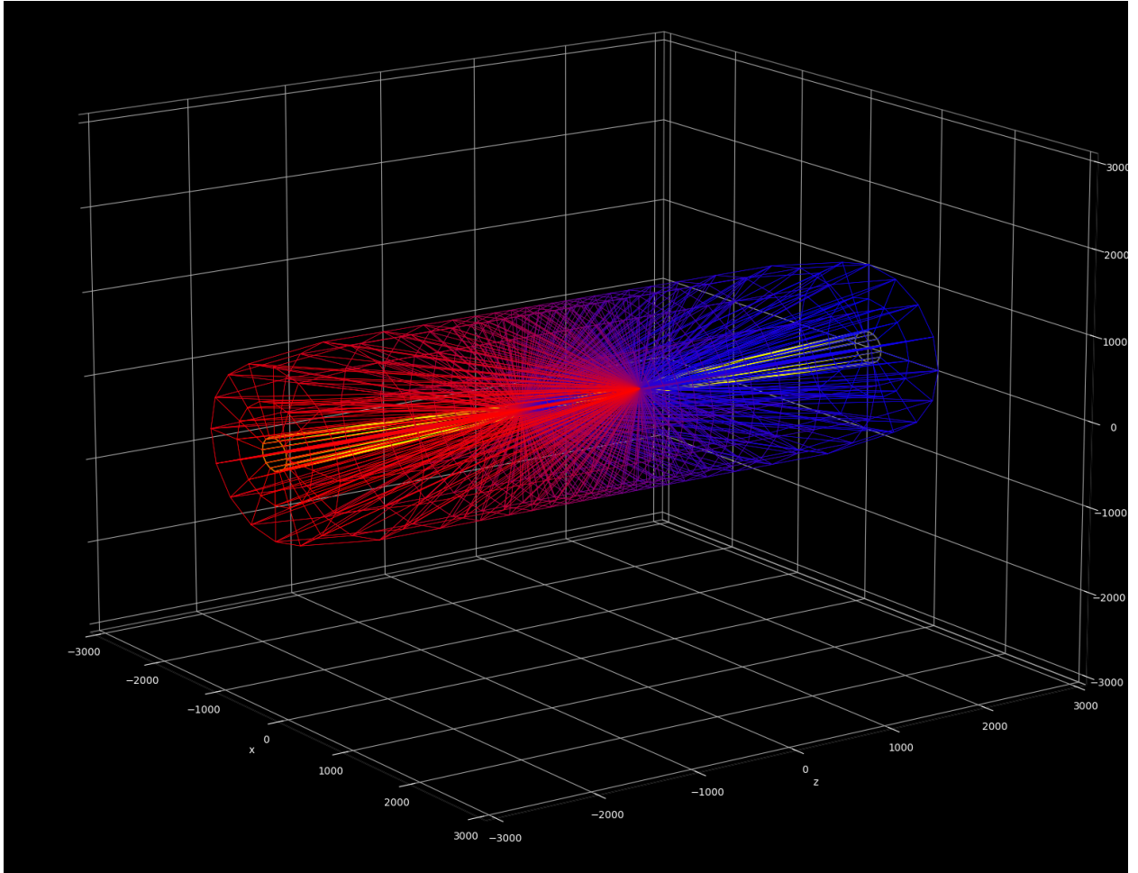
Figure 17: Splitter regions visualization. Pole regions are colored in yellow, wedges are colored with a blue-to-red gradient based on x_{angle} .
