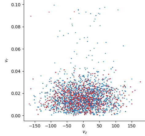
Origin position of found (blue) and missed (red) particles in zr plane
