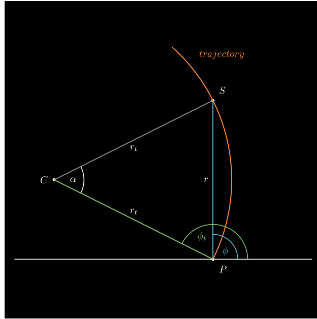
Figure 10: Trajectory and spacepoint in xy plane.
