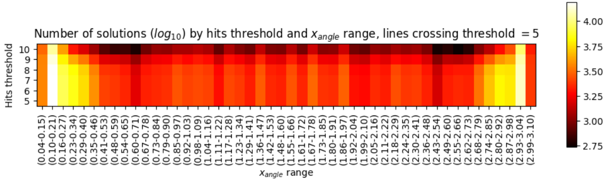
Figure 34: S test: number of solutions heatmaps for hits threshold and x_{angle} ranges with lines crossing threshold = 5.
