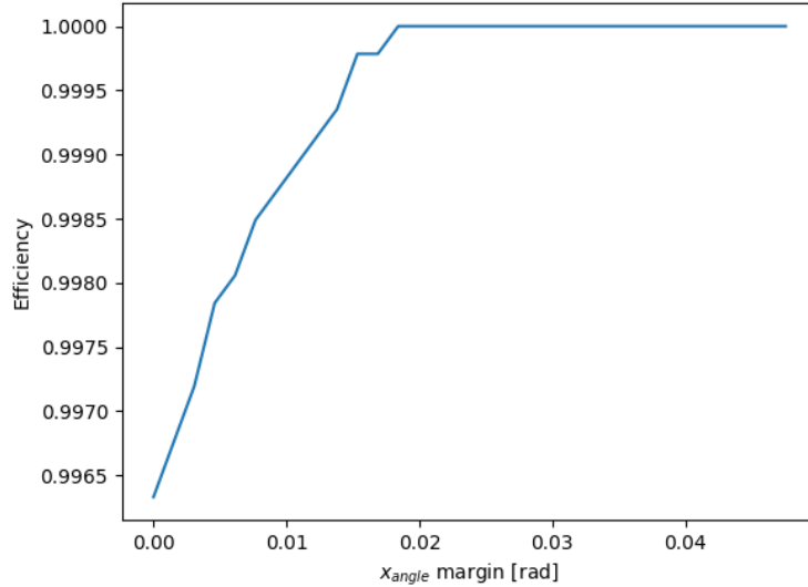
Figure 24: RPPI test: efficiency of finding solutions by x_{angle} margin.
