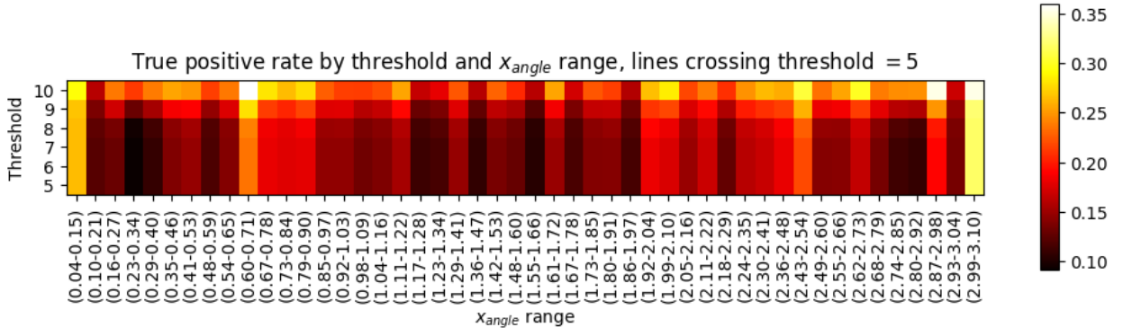
Figure 37: S test: TPR heatmaps for hits threshold and x_{angle} ranges with lines crossing threshold = 5.
