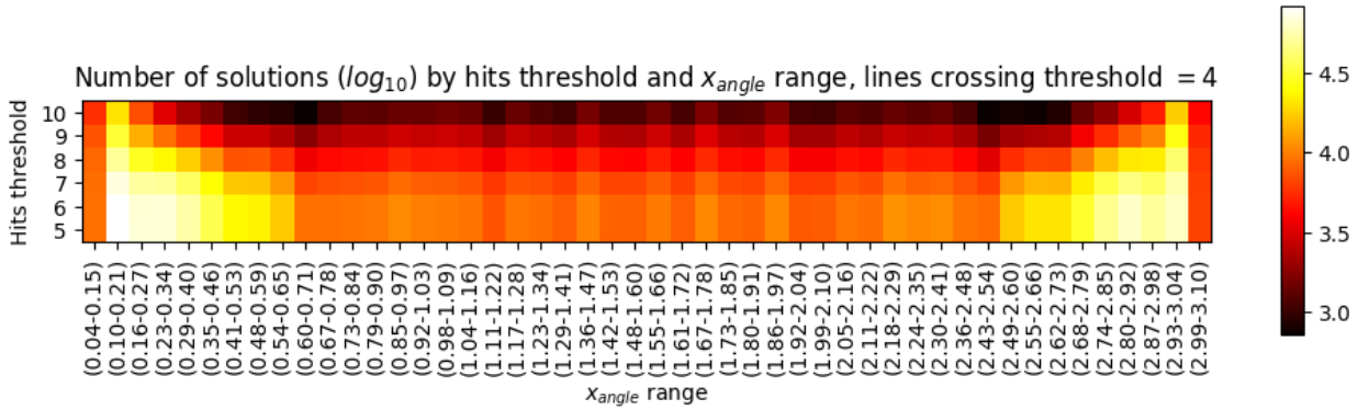
Figure 33: S test: number of solutions heatmaps for hits threshold and x_{angle} ranges with lines crossing threshold = 4.
