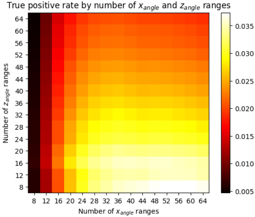
Figure 28: PI test: TPR heatmap for x_{angle} and z_{angle} ranges.
