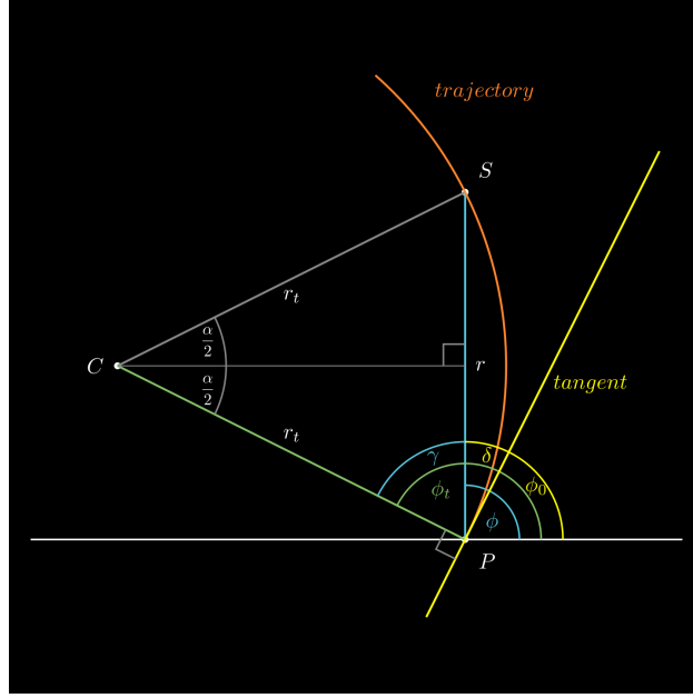
Figure 11: Trajectory and spacepoint in xy plane with tangent.
