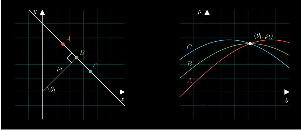
Figure 8: Collinear points in original and Hough spaces.
