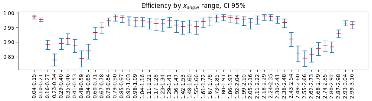
Figure 39: S test: efficiency for custom hits thresholds and lines crossing threshold 4.
