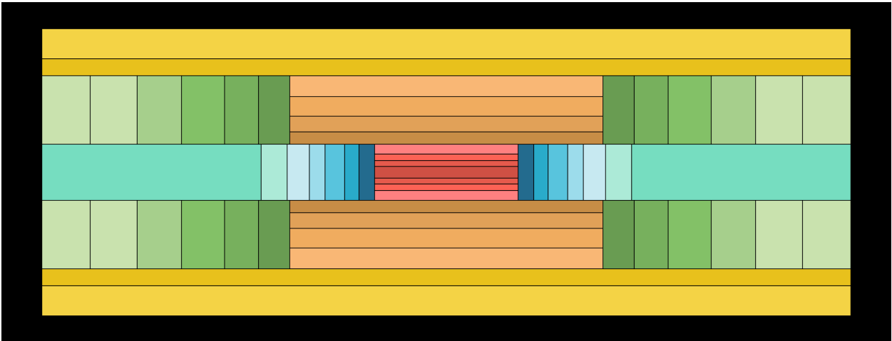
Figure 18: Detector layers in rz plane projection with color-coded groups.
