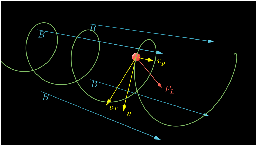
Figure 3: Movement of an electrically charged particle in a magnetic field.
