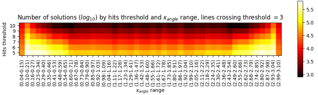
Figure 32: S test: number of solutions heatmaps for hits threshold and x_{angle} ranges with lines crossing threshold = 3.
