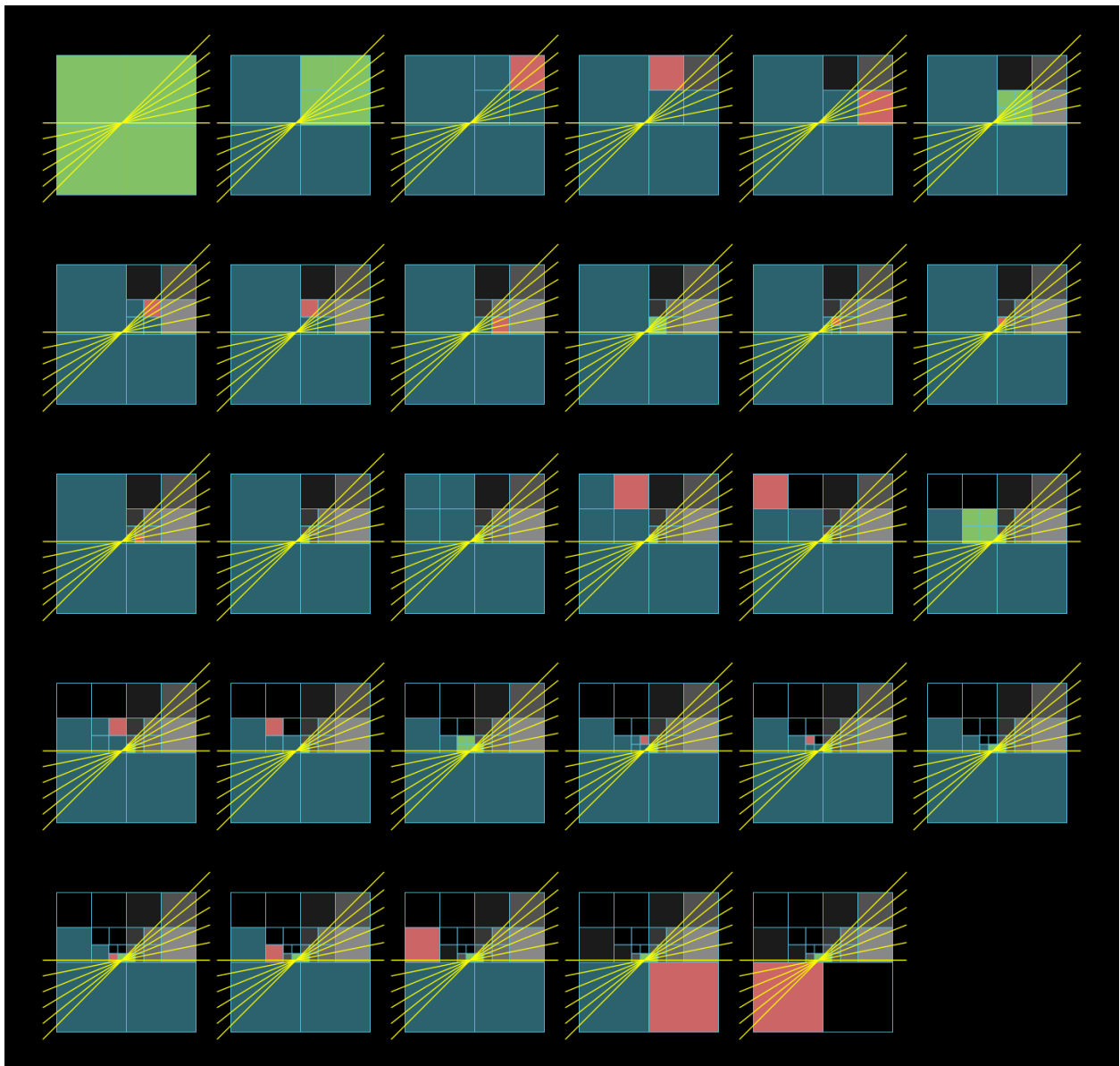
Figure 12: Filling of the accumulator in subsequent cycles of the algorithm.
