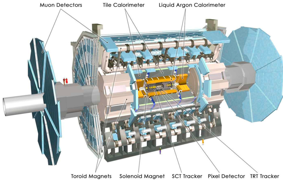
Figure 1: ATLAS detector with the subdetector components. Source: [Gaz24]
