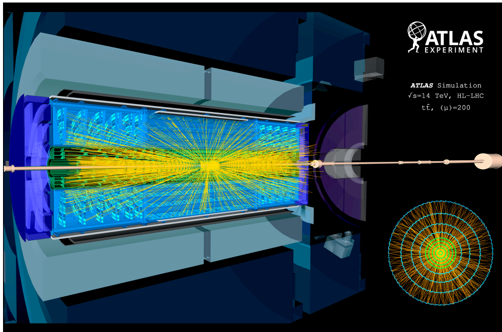
Figure 2: ATLAS HL-LHC bunch crossing simulation with pile-up \mu = 200 . Source: [23]
