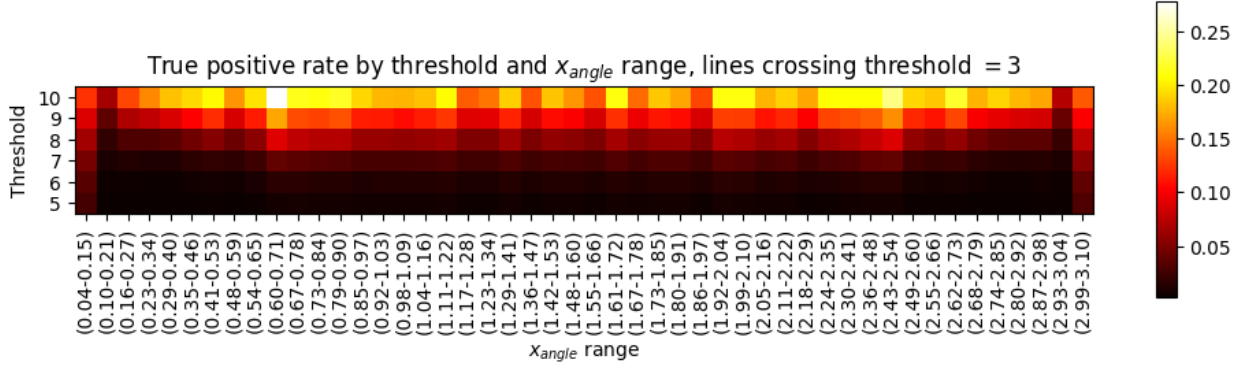
Figure 35: S test: TPR heatmaps for hits threshold and x_{angle} ranges with lines crossing threshold = 3.
