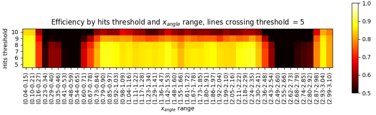
Figure 31: S test: efficiency heatmaps for hits threshold and x_{angle} ranges with lines crossing threshold = 5.
