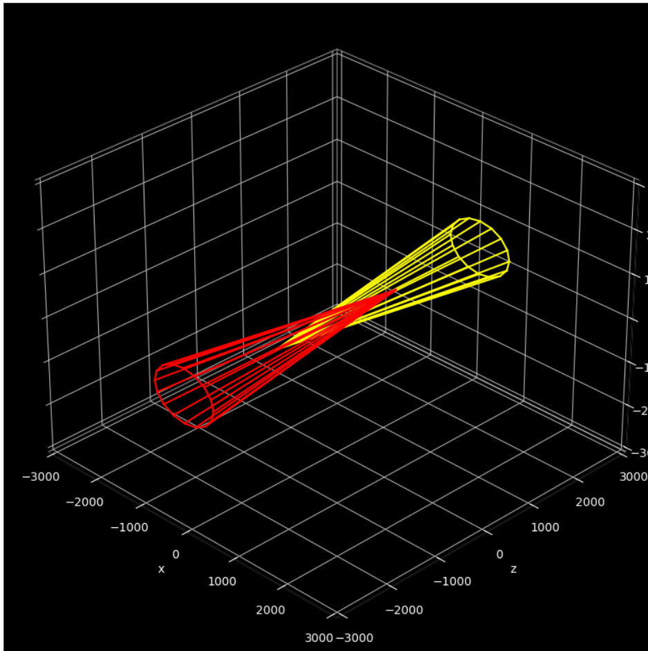
Figure 16: Pole regions.
