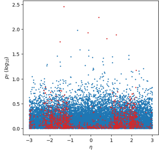
\eta and p_T ( \log_{10} ) of found (blue) and missed (red) particles
