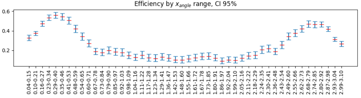
Figure 43: S test: accidental efficiency for custom hits thresholds and lines crossing threshold 4.
