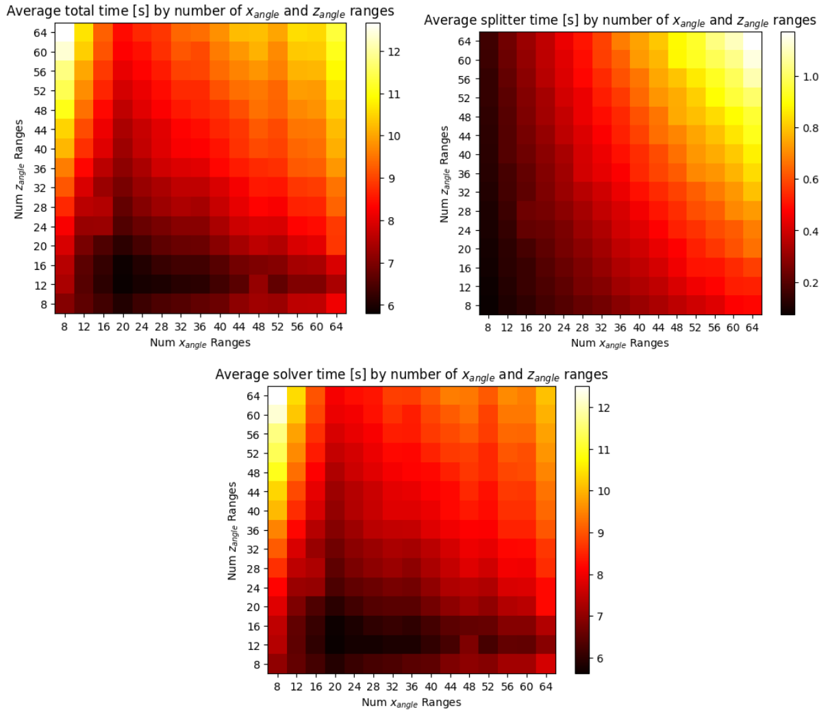
Figure 45: S test: execution times by number of x_{angle} and z_{angle} ranges.
