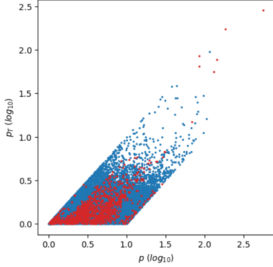
p and p_T of found (blue) and missed (red) particles
