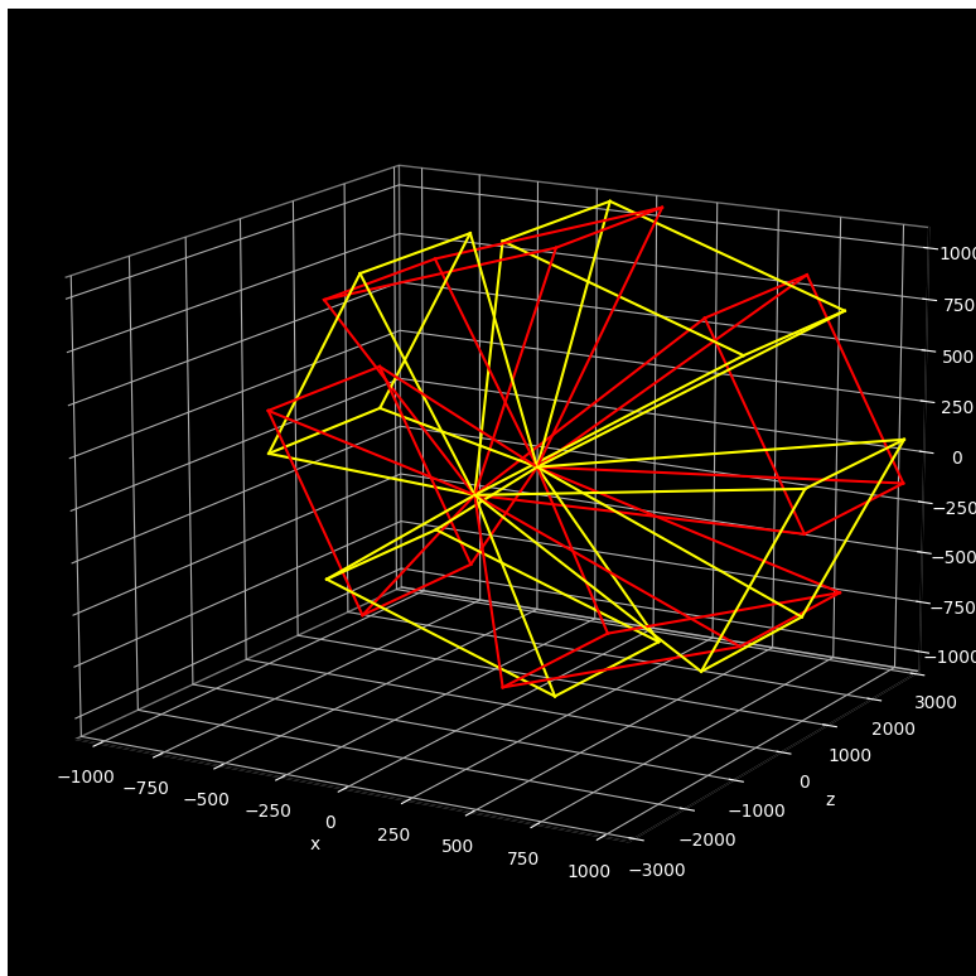
Figure 14: 8 overlapping wedges around z -axis colored in red and yellow.
