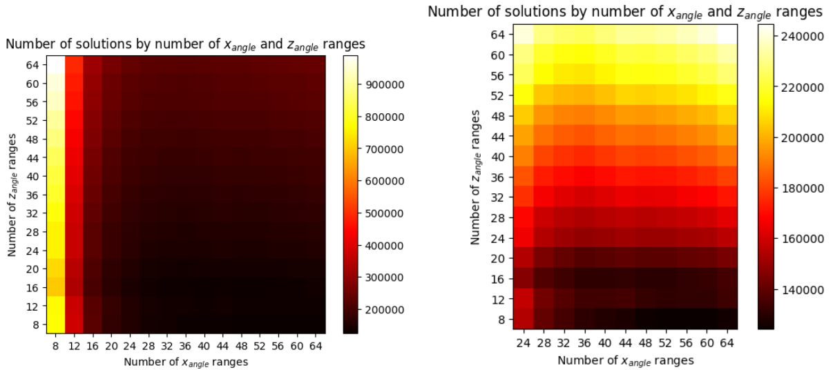
Figure 27: PI test: number of solutions heatmap for x_{angle} and z_{angle} ranges.
