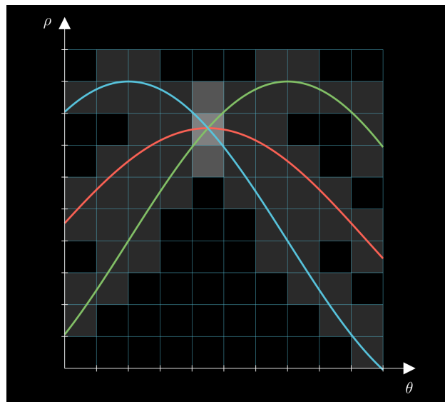
Figure 9: Hough accumulator filling example with 3 points.
